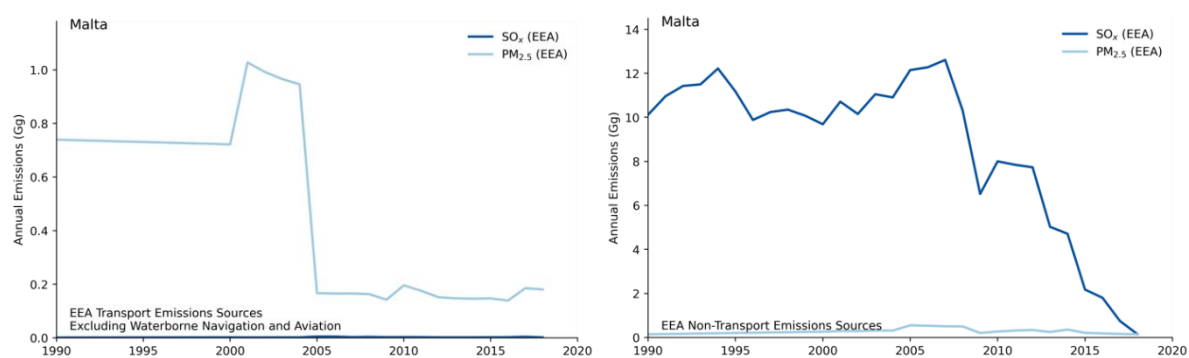
Figure 8.3-29: Transport (left) and non-transport (right) emissions of \text{SO}_x and \text{PM}_{2.5} in Malta
