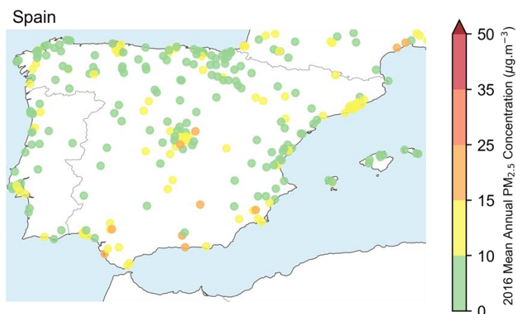
Figure 8.3-42: WHO mean annual \text{PM}_{2.5} concentration observations in Spain (2016)
