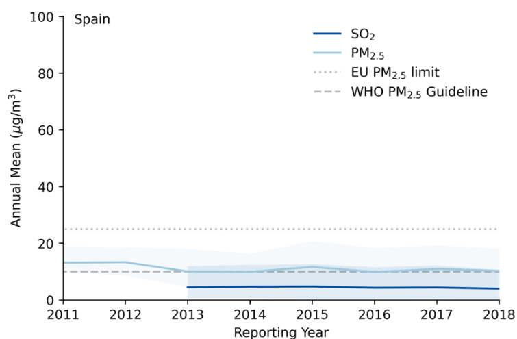
Figure 8.3-41: Annual mean concentrations of \text{SO}_2 and \text{PM}_{2.5} in Spain (shaded areas show 95% CI)
