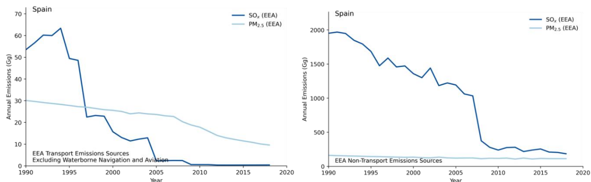
Figure 8.3-40: Transport (left) and non-transport (right) emissions of \text{SO}_x and \text{PM}_{2.5} in Spain
