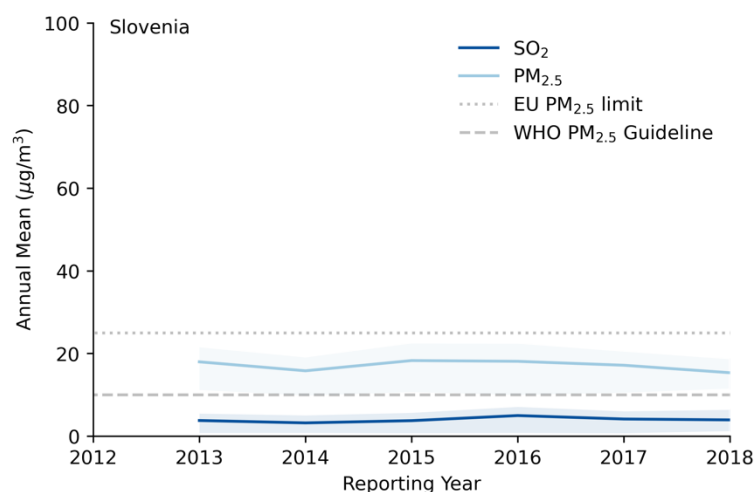
Figure 8.3-38: Annual mean concentrations of \text{SO}_2 and \text{PM}_{2.5} in Slovenia (shaded areas show 95% CI)
