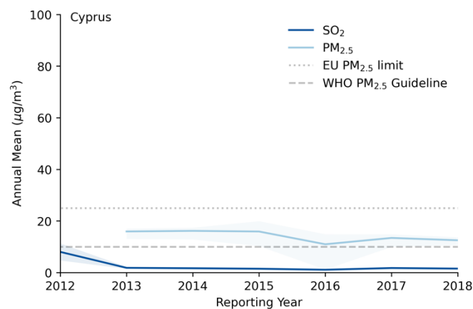
Figure 8.3-14: Annual mean concentrations of SO_2 and PM_{2.5} in Cyprus (shaded areas show
