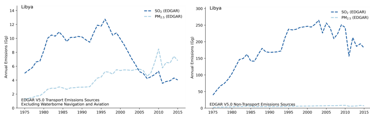
Figure 8.3-28: Transport (left) and non-transport (right) emissions of \text{SO}_2 and \text{PM}_{2.5} in Libya
