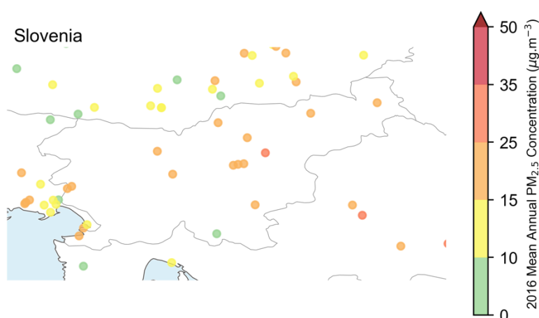
Figure 8.3-39: WHO mean annual \text{PM}_{2.5} concentration observations in Slovenia (2016)
