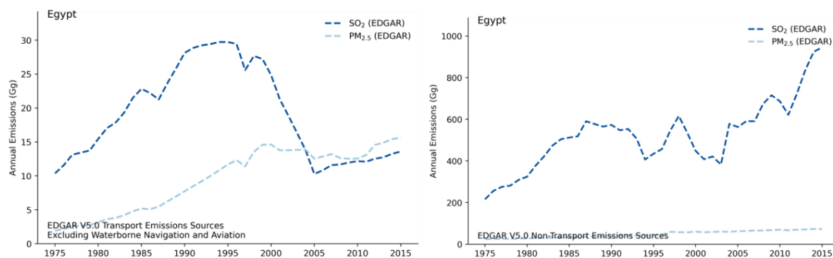
Figure 8.3-16: Transport (left) and non-transport (right) emissions of \text{SO}_2 and \text{PM}_{2.5} in Egypt
