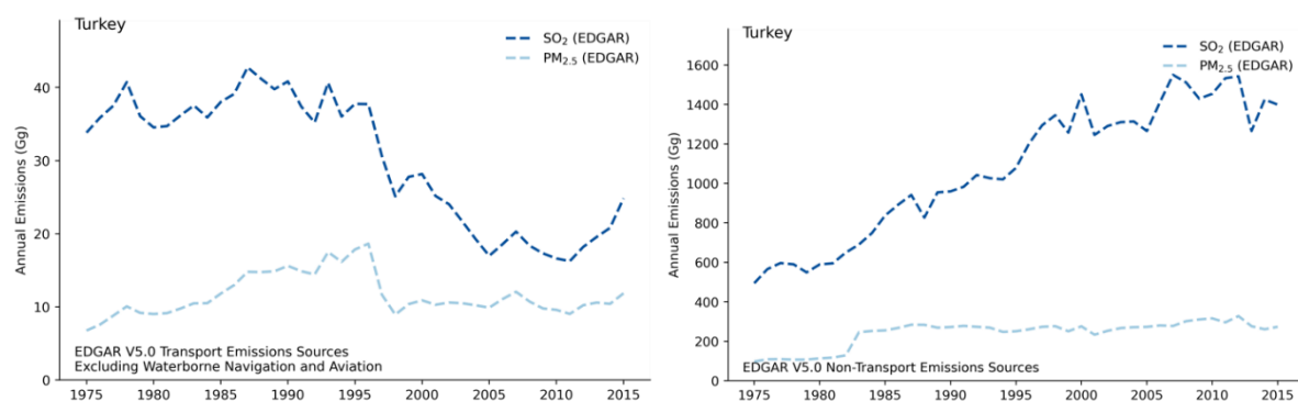
Figure 8.3-45: Transport (left) and non-transport (right) emissions of \text{SO}_2 and \text{PM}_{2.5} in Turkey
