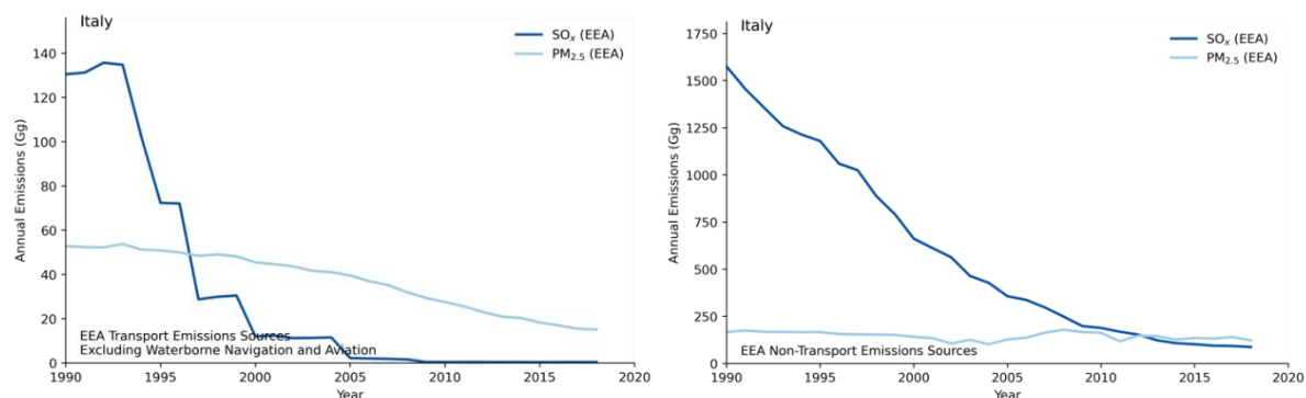
Figure 8.3-24: Transport (left) and non-transport (right) emissions of \text{SO}_x and \text{PM}_{2.5} in Italy
