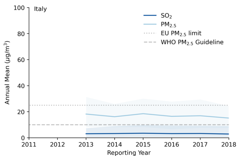
Figure 8.3-25: Annual mean concentrations of \text{SO}_2 and \text{PM}_{2.5} in Italy (shaded areas show 95% CI)
