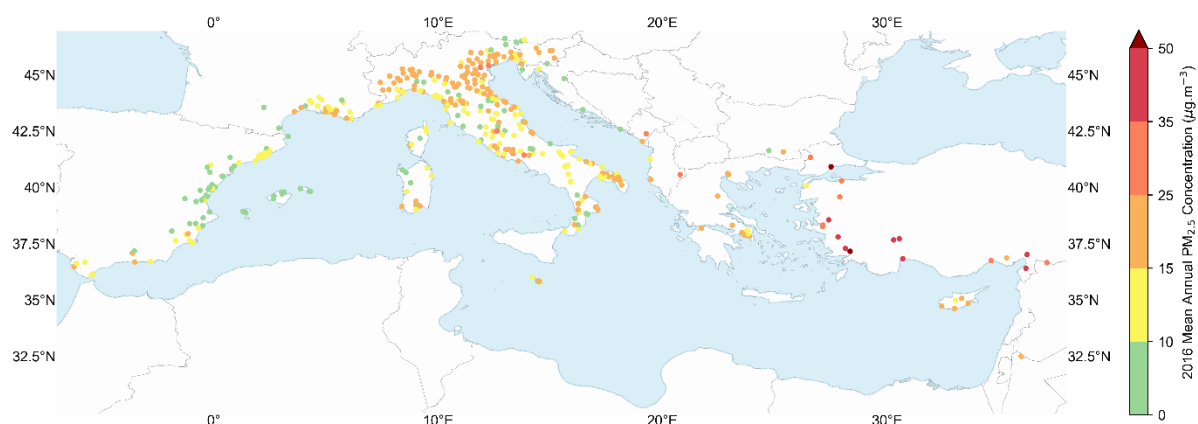
Figure 8.3-3: Mean annual air quality ( PM_{2.5} \mu\text{g}/\text{m}^3 ) observed at coastal observation stations (within 100 km of the coastline)
