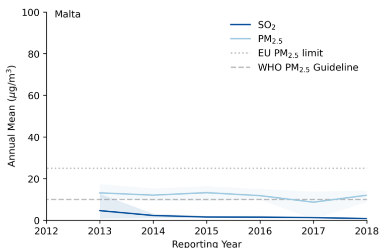
Figure 8.3-30: Annual mean concentrations of \text{SO}_2 and \text{PM}_{2.5} in Malta (shaded areas show
