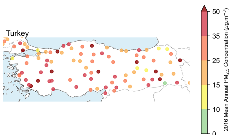
Figure 8.3-46: WHO mean annual \text{PM}_{2.5} concentration observations in Turkey (2016)
